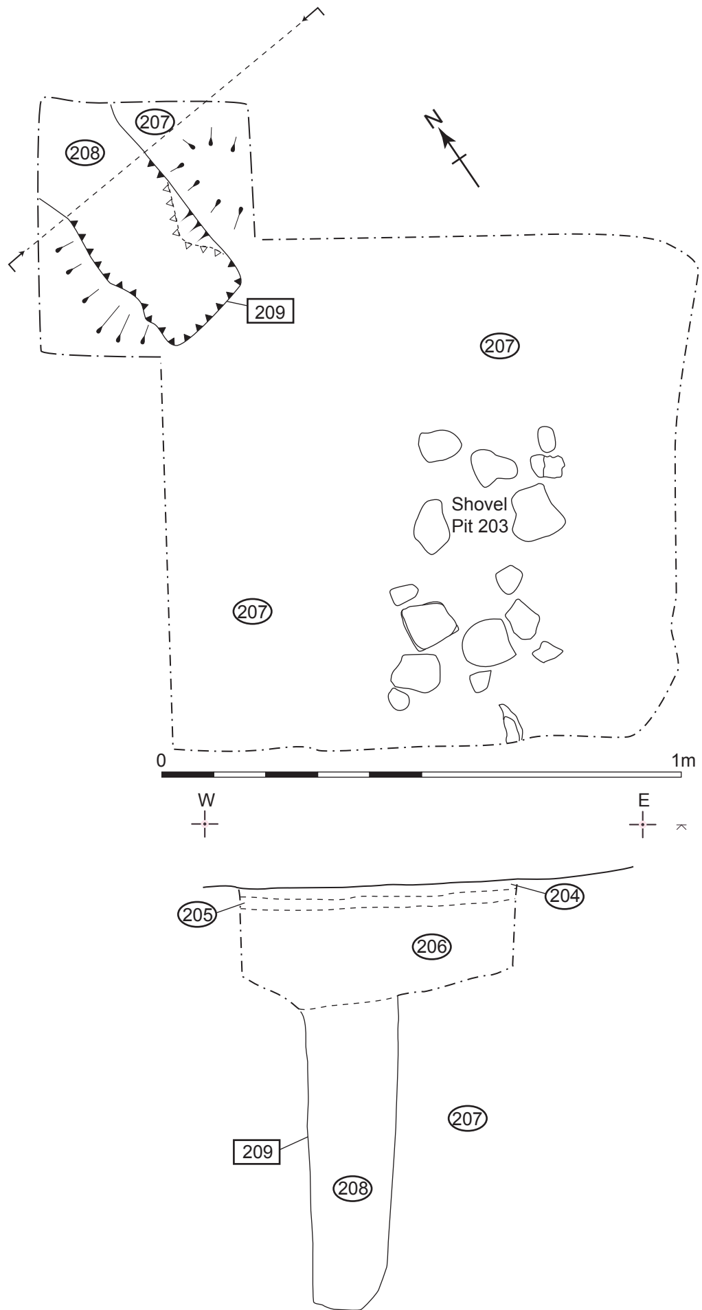
Figure 18 Peat Moss / Wetherhouse Moor Test Pit 2, plan and south facing section
